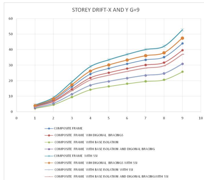
Graph 4.2- Storey Drift-X & Y Direction
