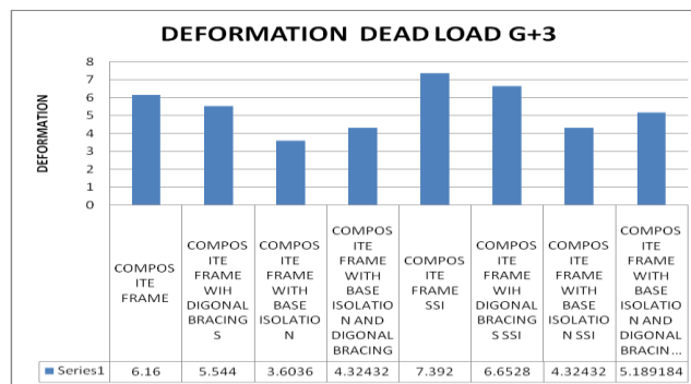
Graph 4.4: Deformation Dead Load
