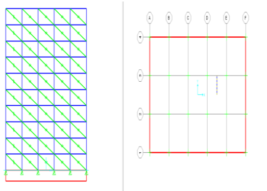
Fig 3.3 Plan and Elevation on sap 2000
