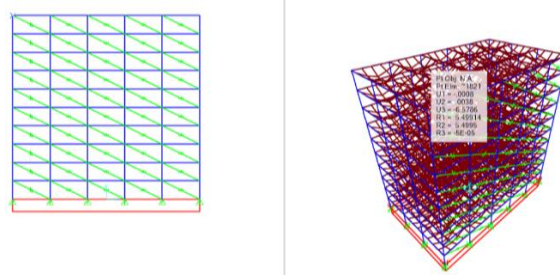
Fig 3.3 2d and 3d modeling
