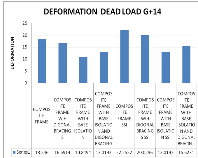
Graph 4.7: Deformation Dead Load
