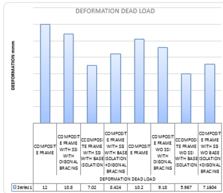
Graph 4.1: Deformation Dead Load G+9
