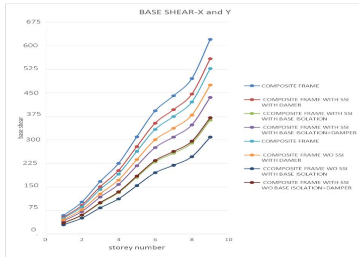
Graph 4.3: Base shear along x and y direction
