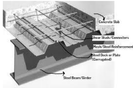
Fig 1.2: Composite deck slab and beams
