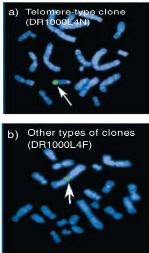
Figure 2 to be located in chromosomal DNA by FISH. (a) Genes near the telomeric region that are amplified. There are genes on other chromosomes that have been amplified. The white arrow indicates the site of the amplified genes, and the count terstaining was performed using DAP
