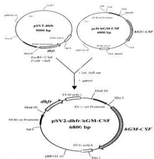
Figure 1. The process of creating the pSV2-dhfr/hGM CSF vector. From the pSV2-dhfr and pcD-hGM-CSF vectors, a pSV2-dhfr/hGM-CSF vector was created There was a tandem arrangement of the Dhfr and hGM-CSF genes on this plasmid, and the SV40 ori promoter and SV40 polyA terminator were necessary to calculate the specific growth and human GM-CSF production rates (per cell per hour) with 95% confidence level. As a result of the findings, the level of confidence is less than 5% of the rates. It was determined using a 96-well plate enzyme-linked immunosorbent
